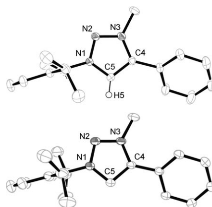
Figure 1. Molecular views (thermal ellipsoids set at 50% probability) of 2a (top) and Va (bottom) in the solid state. For clarity, counterions, solvent molecules, and H atoms are omitted, except for the ring hydrogen of 2a . Selected bond lengths [Å] and angles [°] for 2a : N1–N2 1.3208(16), N2–N3 1.3183(16), N3–C4 1.3559(17), C4–C5 1.3647(19), C5–N1 1.3446(17); N1–C5–C4 105.85(12). Va : N1–N2 1.3439(12), N2–N3 1.3216(13), N3–C4 1.3682(13), C4–C5 1.4053(14), C5–N1 1.3662(13); N1–C5–C4 99.70(8).
